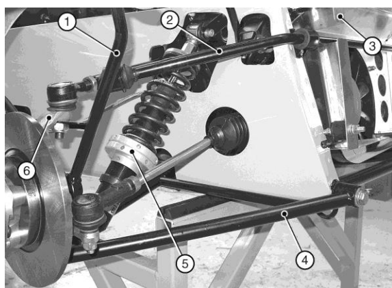
Figure 32: Front suspension
