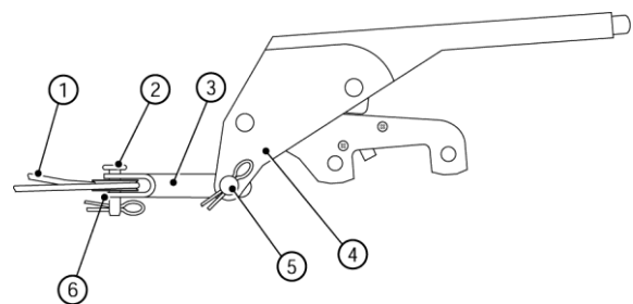
Figure 130: Handbrake assembly
