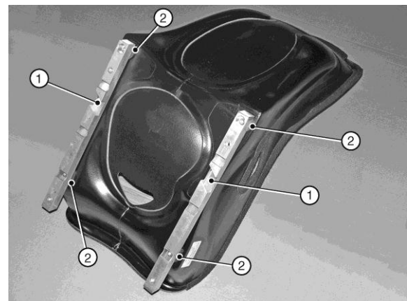
Figure 144: Fixed seat
