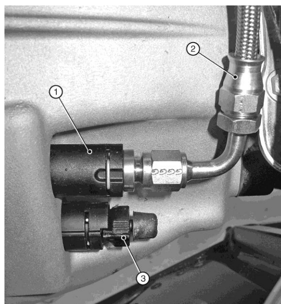
Figure 168: Clutch hydraulic connections
