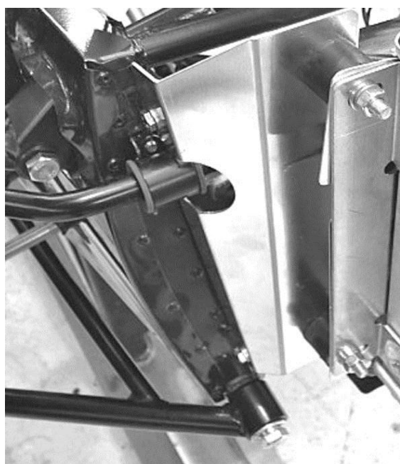
Figure 105: SV radiator arrangement
