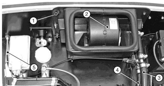
Figure 79: Heater installation
