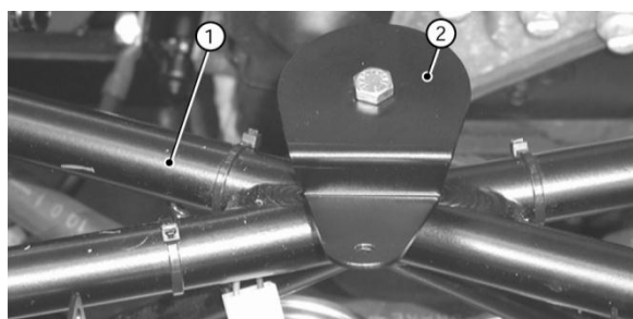
Figure 78: Coolant expansion bottle mounting bracket
