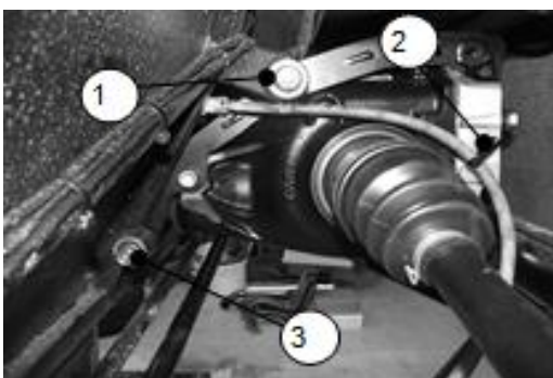
Figure 118: Differential installation and LHS
