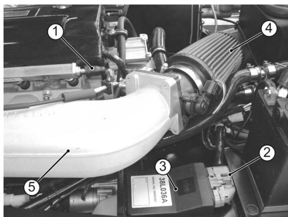
Figure 65: ECU
