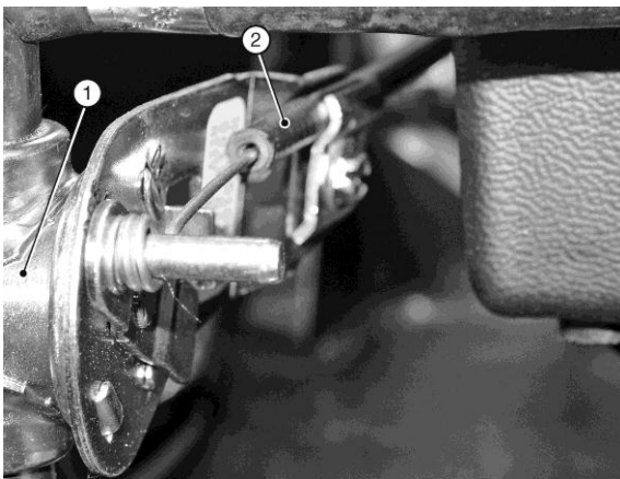
Figure 112: Heater control cable attachment
