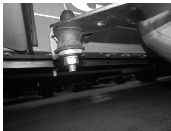
Figure 173: Exhaust mounting
