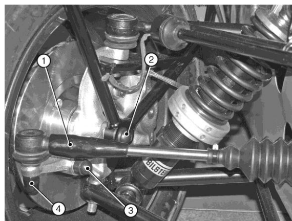
Figure 172: Front suspension
