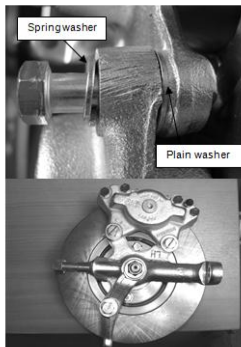
Figure 209: Front brake calliper assembly
