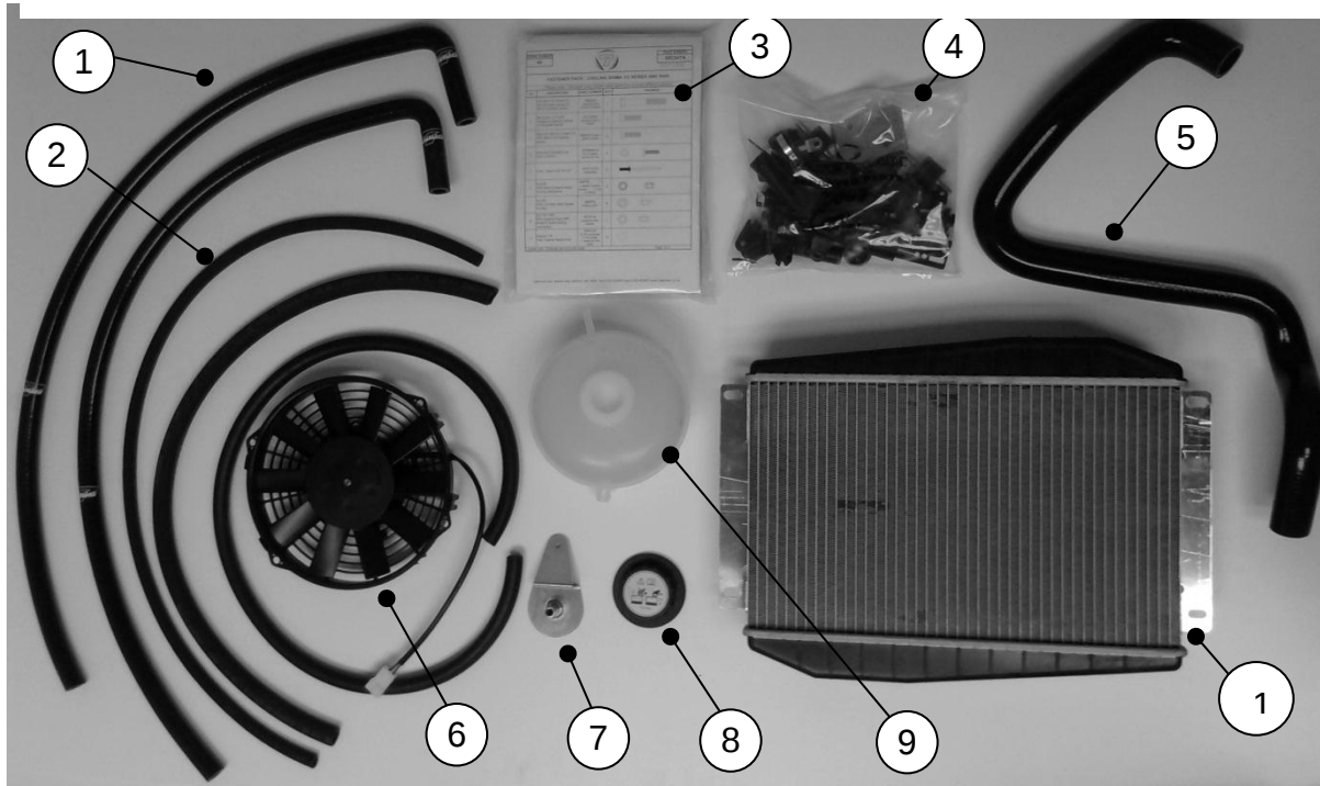
Figure 7: Cooling items
