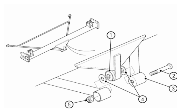
Figure 124: Metalistic brush - De Dion tube
