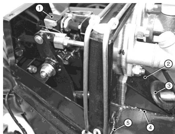
Figure 66: Brake light switch harness
