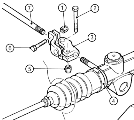
Figure 26: Steering rack to steering column
