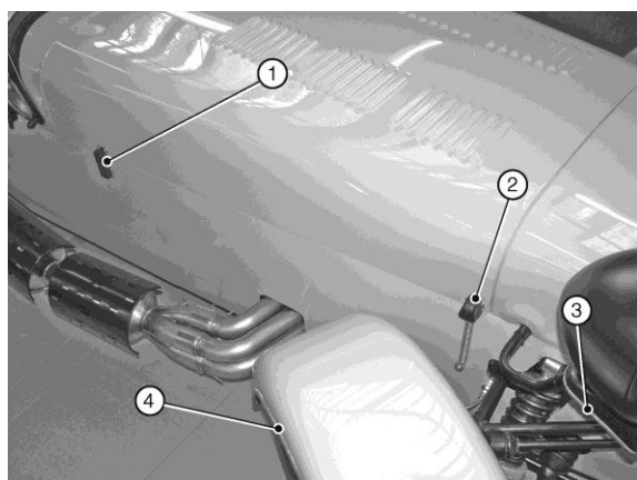
Figure 171: Bonnet catches
