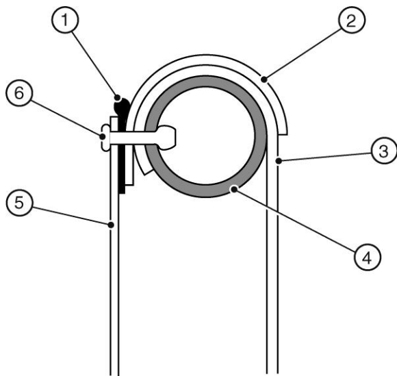
Figure 136: Trim fixings
