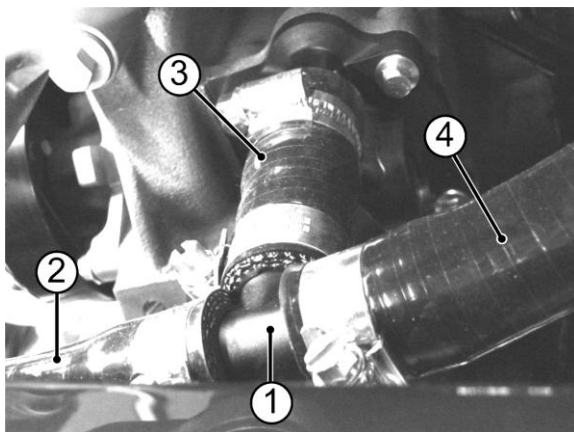
Figure 80: Coolant hoses
