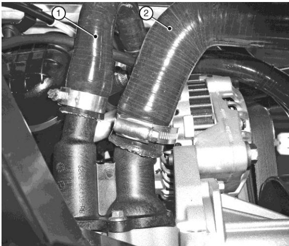
Figure 48: Bottom hose engine connection (viewed from bellow)
