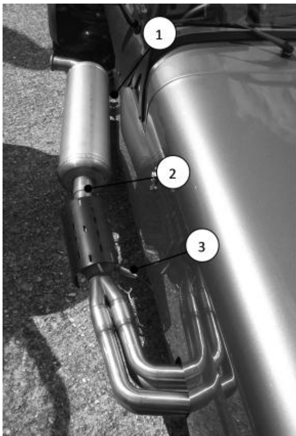
Figure 73: Exhaust arrangement
